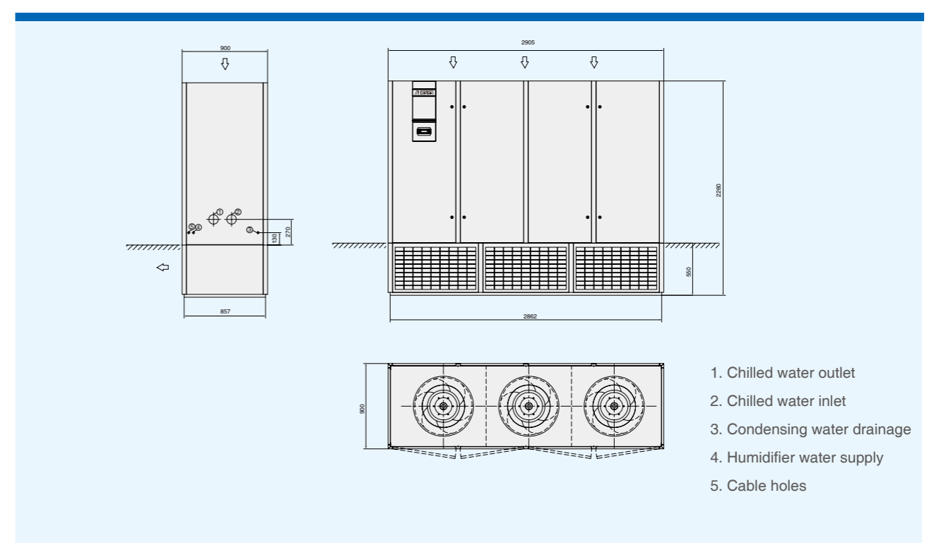
B4 Unit Cabinet Dimension Drawing for Under Flow Unit
