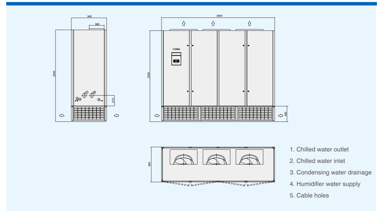
B4 Unit Cabinet Dimension Drawing for Up Flow Unit
