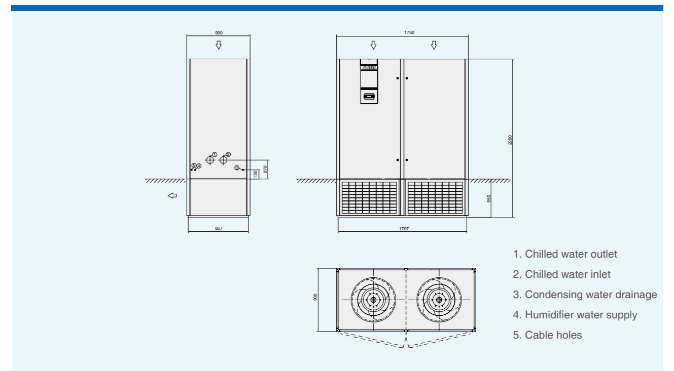
B2 Unit Cabinet Dimension Drawing for Under Flow Unit
