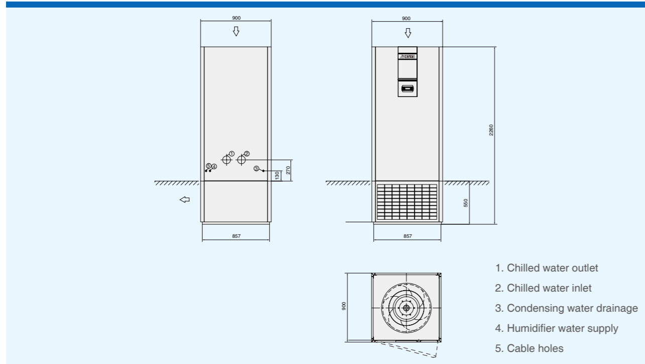
B1 Unit Cabinet Dimension Drawing for Under Flow Unit
