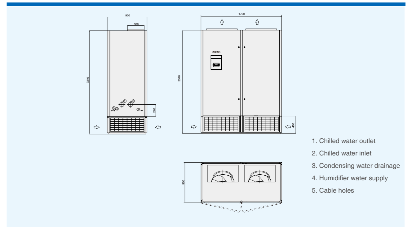
B2 Unit Cabinet Dimension Drawing for Up Flow Unit
